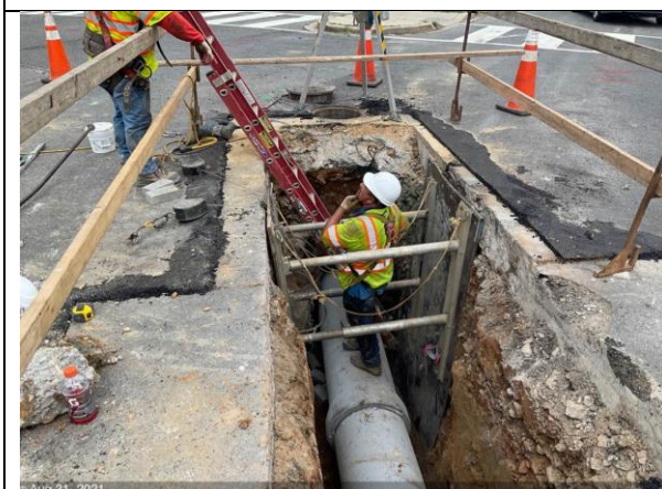
C St NE & 18th St – Place 18" RCP between M6-3 and M6-4
