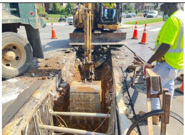
C St NE & 18th St – Trench for RCP between M6-3 and M6-4
