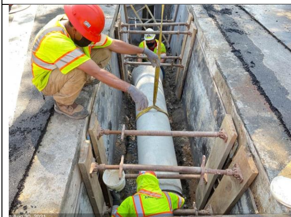
C St NE & 21st St – 15" RCP between M8-4 and I8-7
