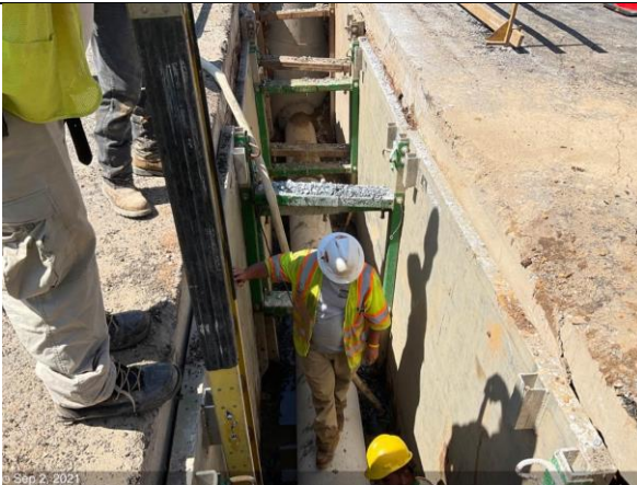
C St NE & 19th St – Verify pipe slope for M6-10 to I7-3
